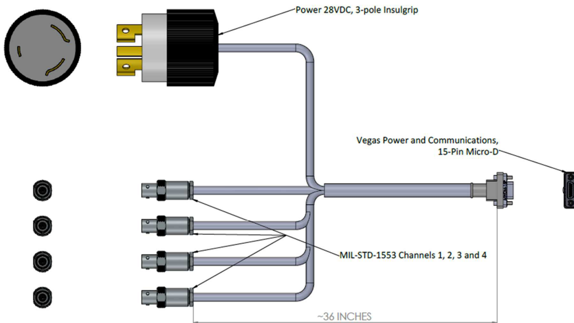
Figure 3: CYB-CBL-02-F Vegas-S Interface Cable
