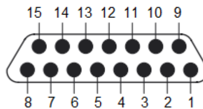
Figure 2: Vegas-S Connector Pin-Out
