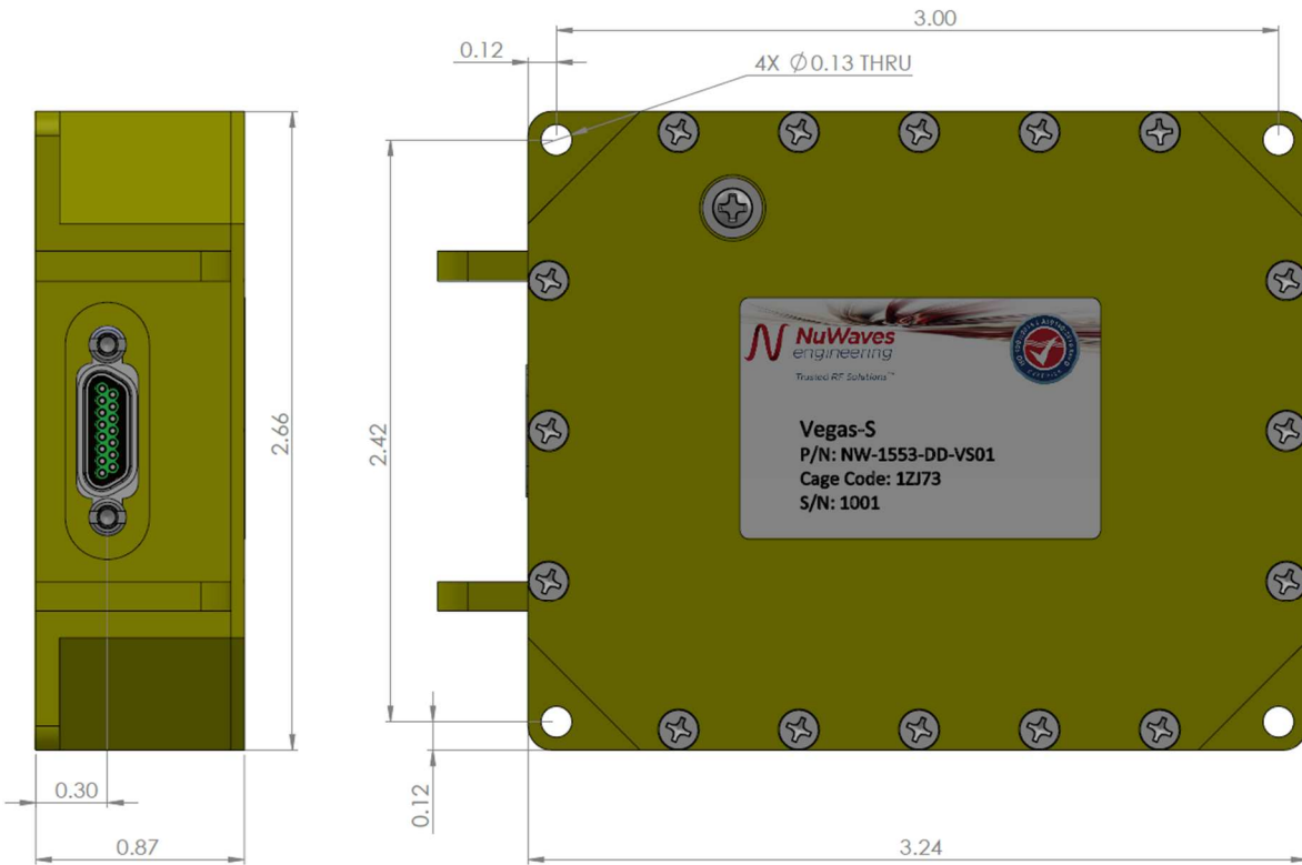
Figure 4: Vegas-S Mechanical Outline
