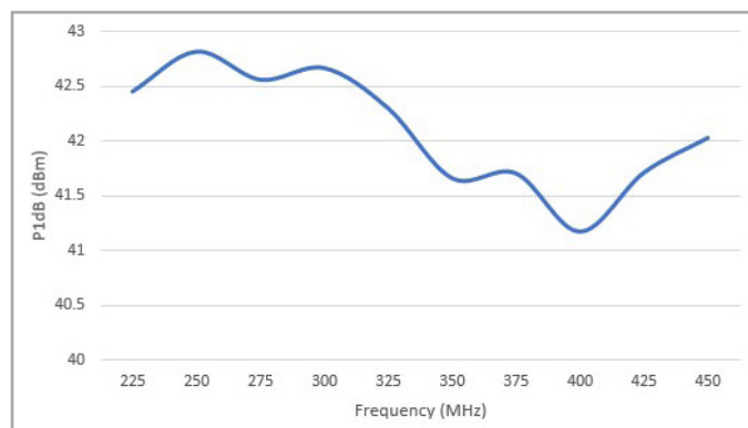
P1dB vs. Frequency
