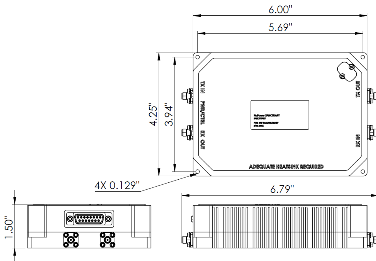
Figure 2: NuPower ULSC-20-C01-S01 Mechanical Outline
