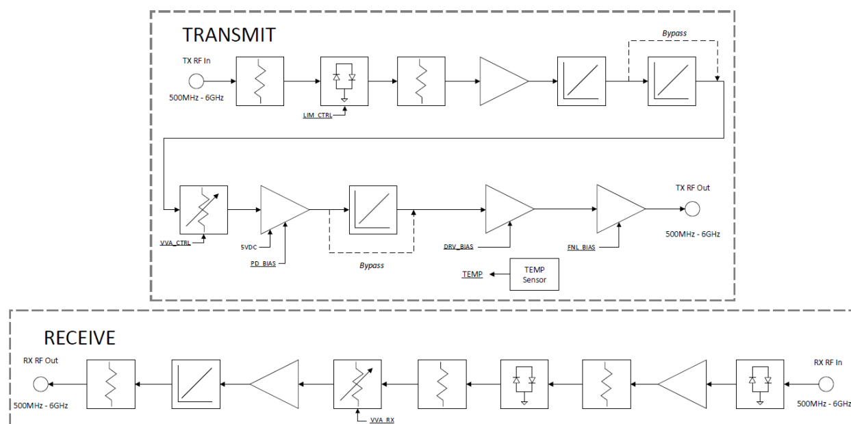
Figure 1: NuPower ULSC-20-C01-S01 Functional Diagram
