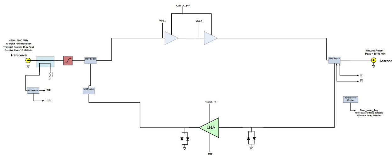
Figure 1: NuPower Xtender C15RX01 Functional Diagram
