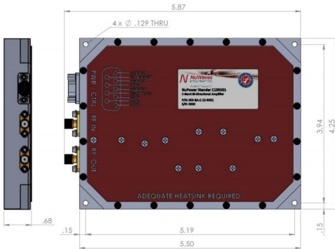
Figure 2: NuPower Xtender C15RX01 Mechanical Outline
