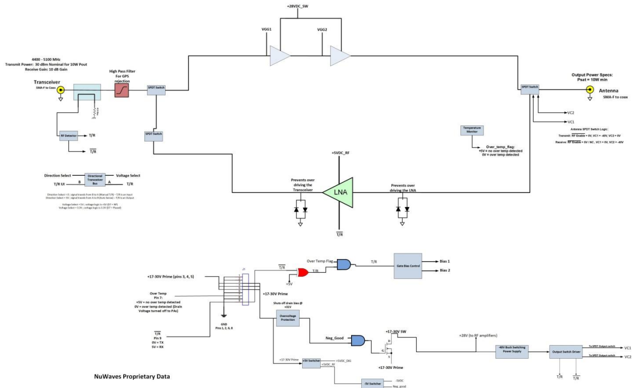
Figure 1: NuPower Xtender C10RX03 Functional Diagram
