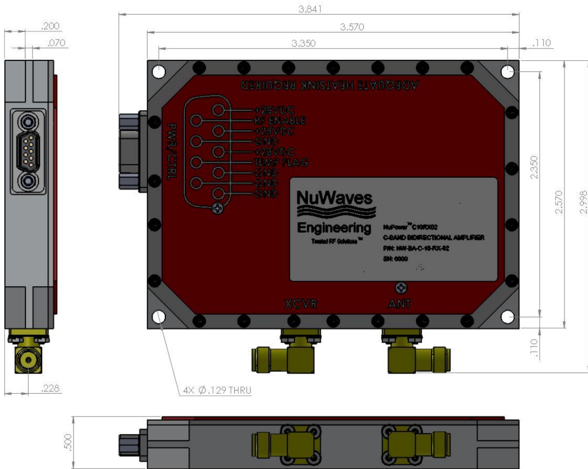
Figure 2: NuPower Xtender C10RX03 Mechanical Outline
