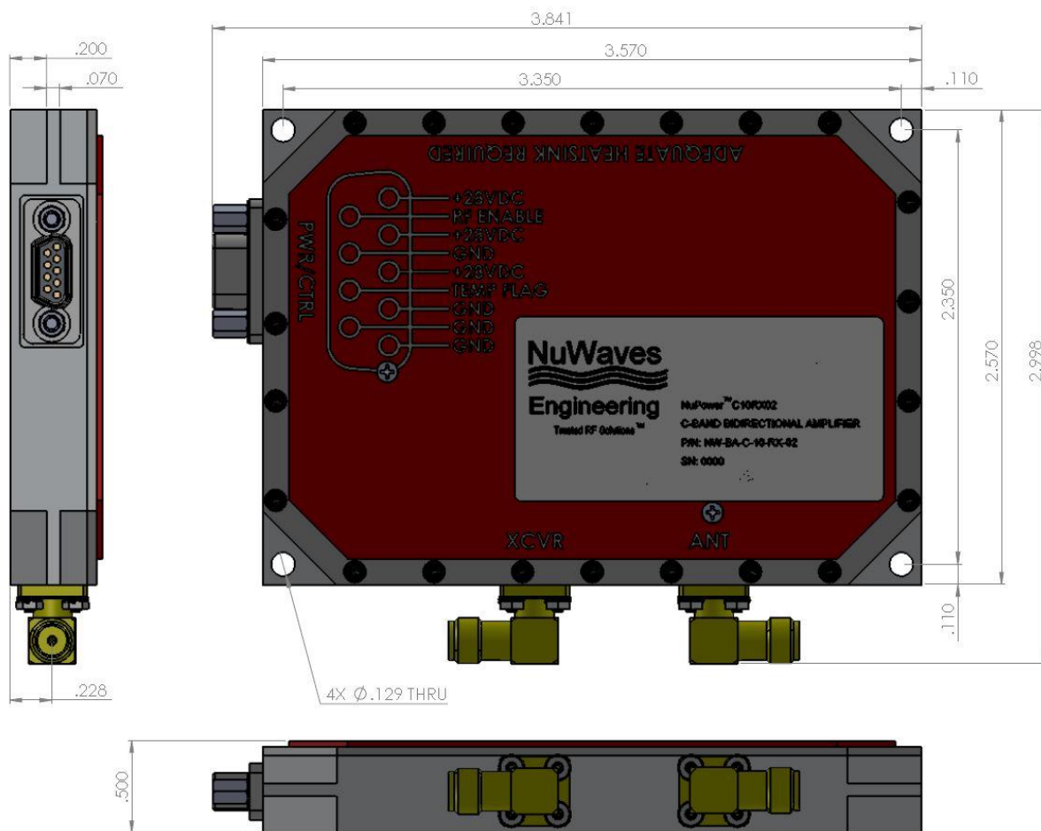
Figure 2: NuPower Xtender C10RX01 Mechanical Outline
