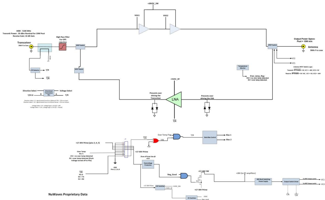
Figure 1: NuPower Xtender C10RX01 Functional Diagram
