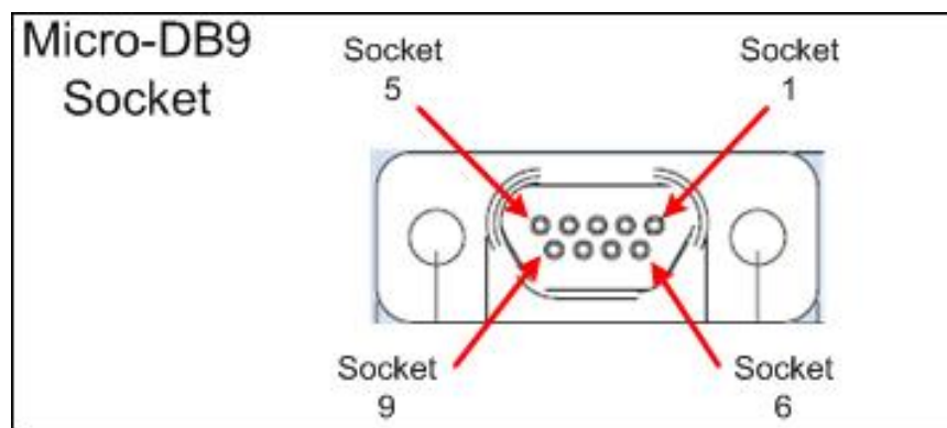
Figure 4: Micro-D Socket Locations
