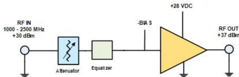
Figure 1: NuPower LS5MI01-D30 Functional Diagram
