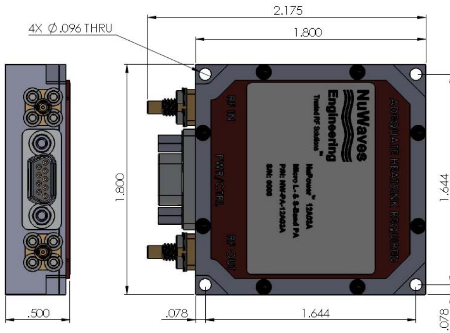
Figure 2: NuPower LS5MI01-D30 Mechanical Outline
