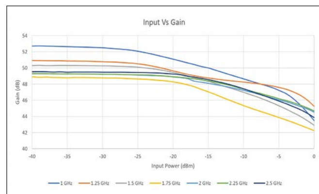
Gain vs. Input Power
