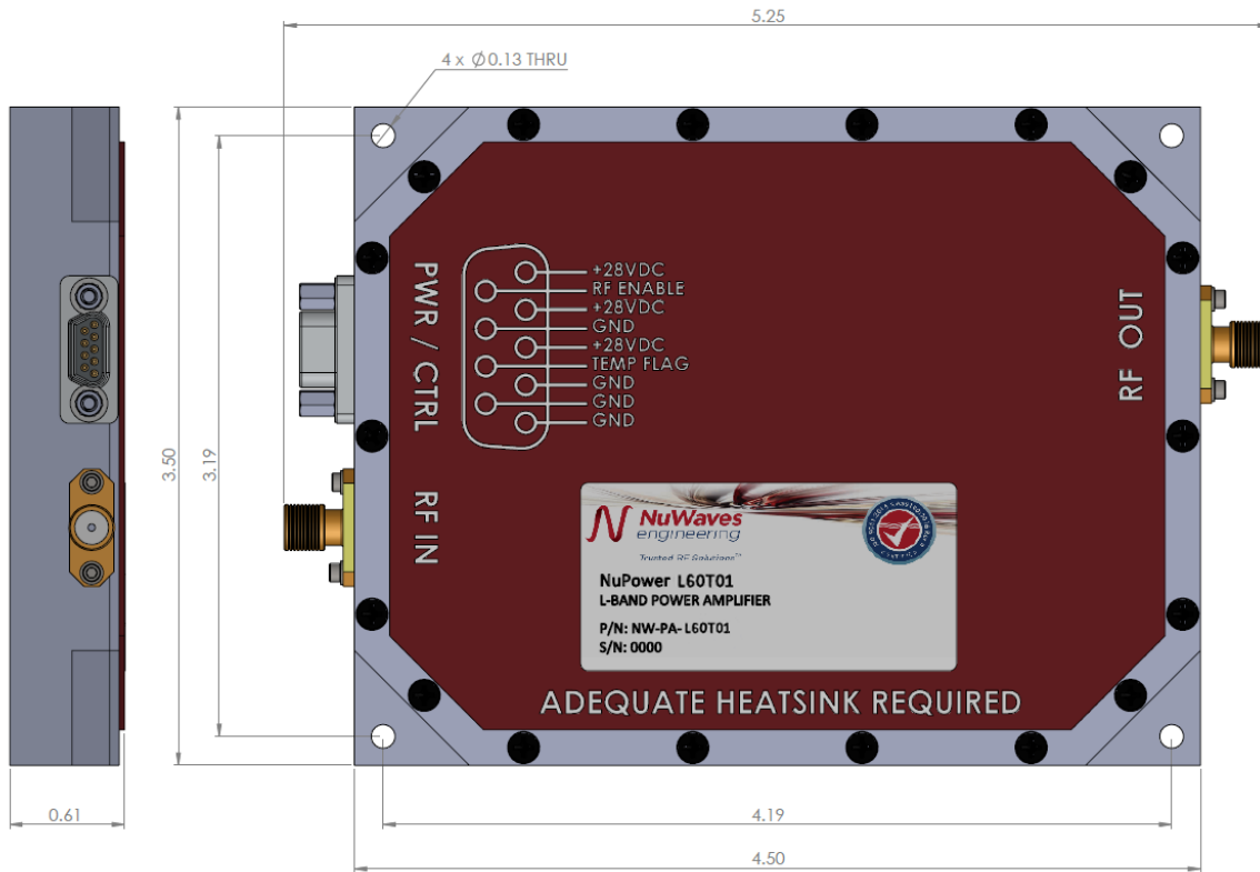
Figure 2: NuPower L60T01 Mechanical Outline
