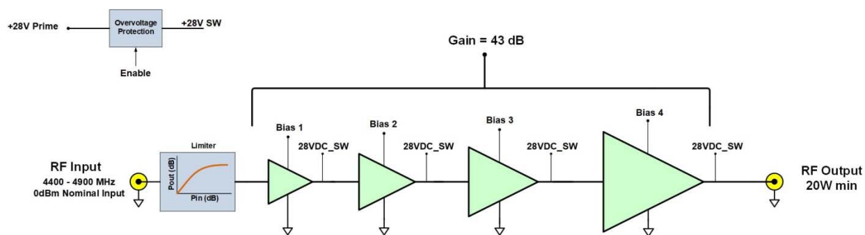
Figure 1: NuPower C20R01 Functional Diagram
