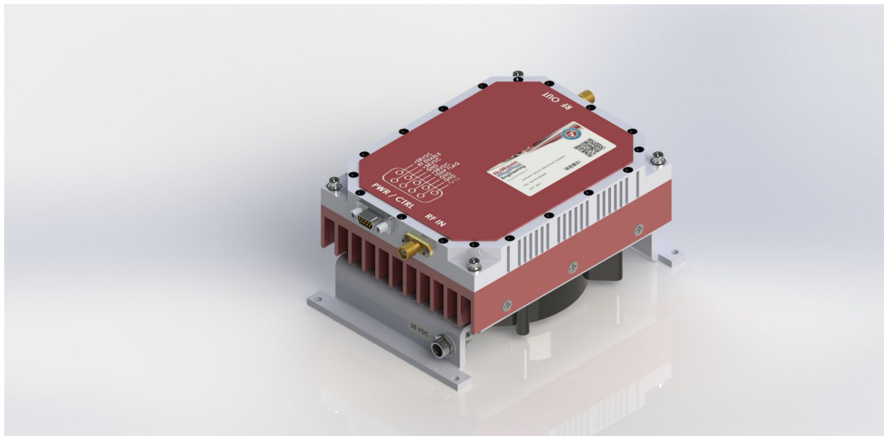
Figure 3: The NuPower PA Kit offers “out-of-the-box” operation for the user. The 28 VDC fan-cooled heatsink is shown with the NuPower C20R01 mounted (the C10R01 is not pictured in this image).
