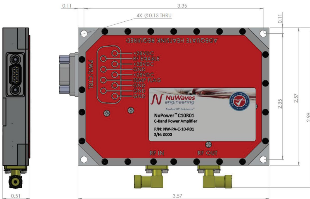
Figure 2: NuPower C10R01 Mechanical Outline
