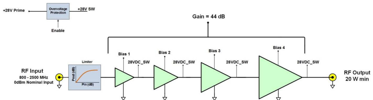
Figure 1: NuPower 15D05A Functional Diagram
