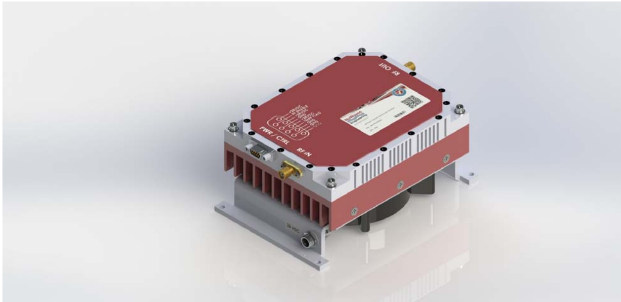
Figure 3: The NuPower PA Kit offers “out-of-the-box” operation for the user. The 28 VDC fan-cooled heatsink is shown with the NuPower 15D05A mounted.
