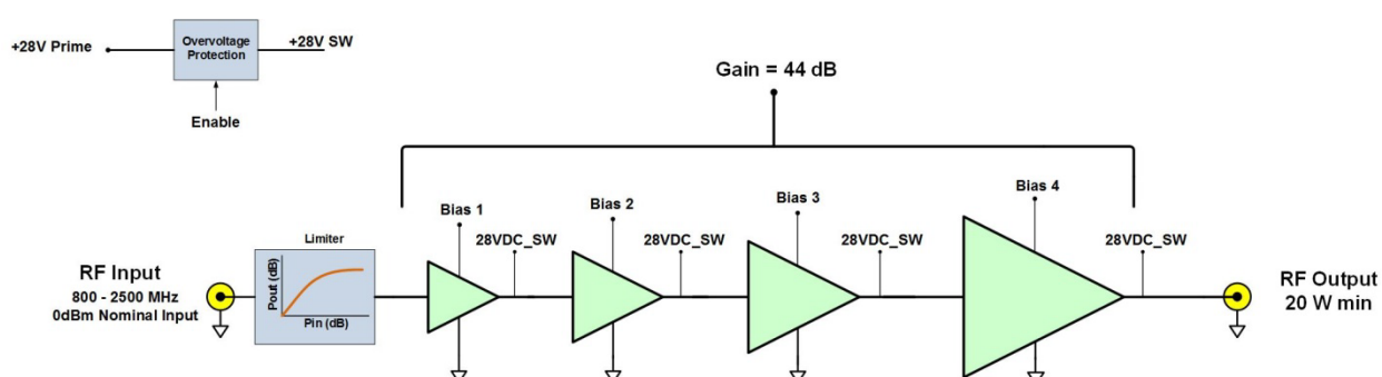
Figure 1: NuPower 15D05A-C01-S01 Functional Diagram
