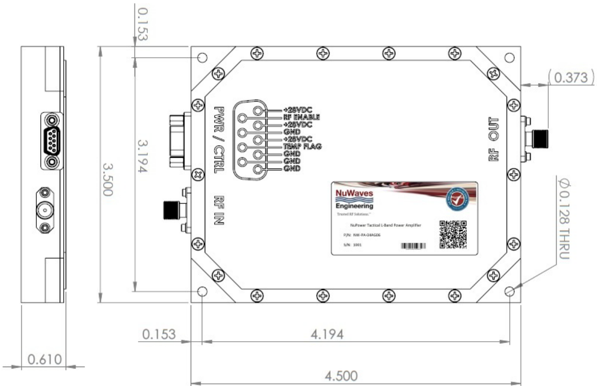
Figure 2: NuPower 15D05A-C01-S01 Mechanical Outline
