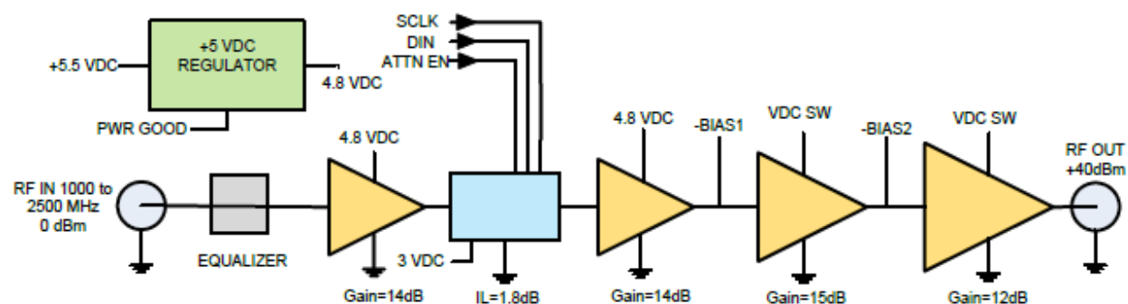
Figure 1: NuPower 12B01A-08 Functional Diagram
