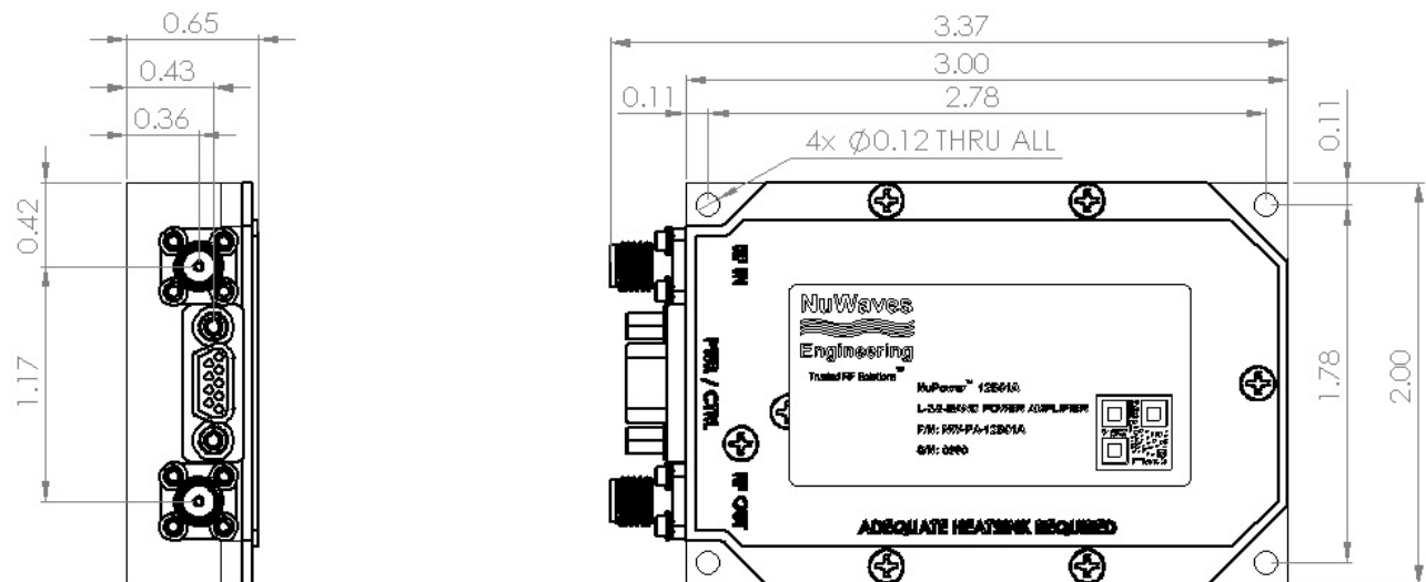
Figure 2: NuPower 12B01A-08 Mechanical Outline
