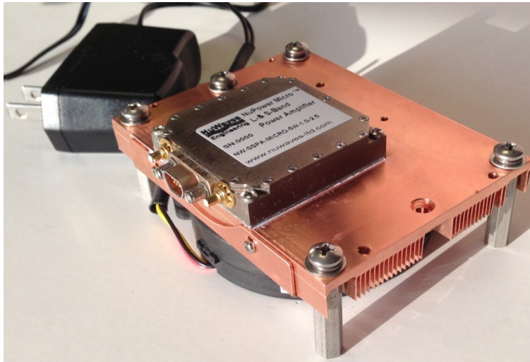
Figure 3: The NuPower PA Kit offers “out-of-the-box” operation for the user. The fan-cooled heatsink with an AC/DC adapter is shown with an example PA (NuPower 12B01A-08 not shown).
