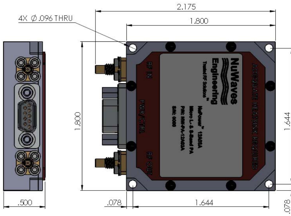
Figure 2: NuPower 12A03A Mechanical Outline
