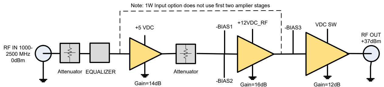
Figure 1: NuPower 12A03A Functional Diagram
