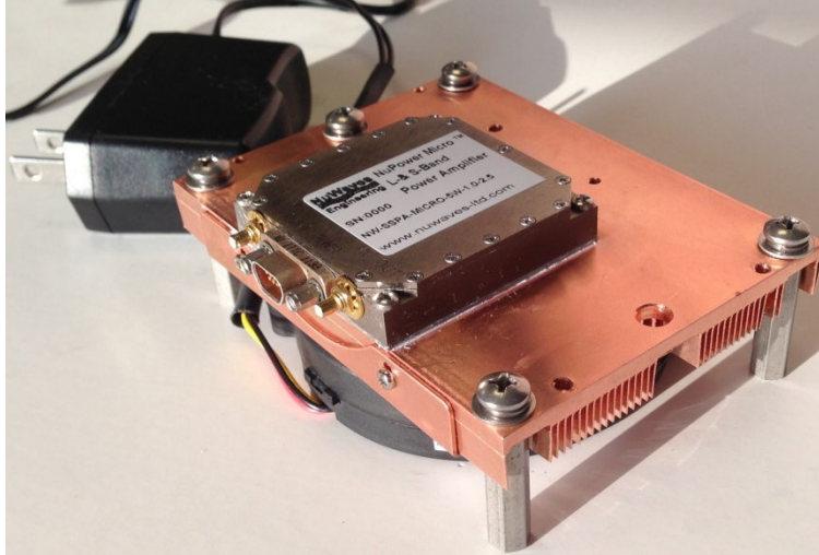
Figure 3: The NuPower PA Kit offers “out-of-the-box” operation for the user. The fan-cooled heatsink with an AC/DC adapter is shown with an example PA (NuPower 12A01A not shown).
