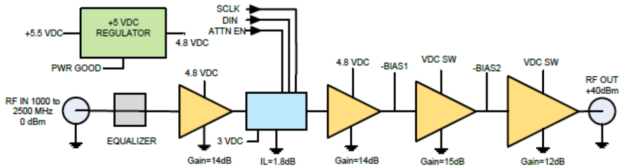
Figure 1: NuPower 12A01A Functional Diagram
