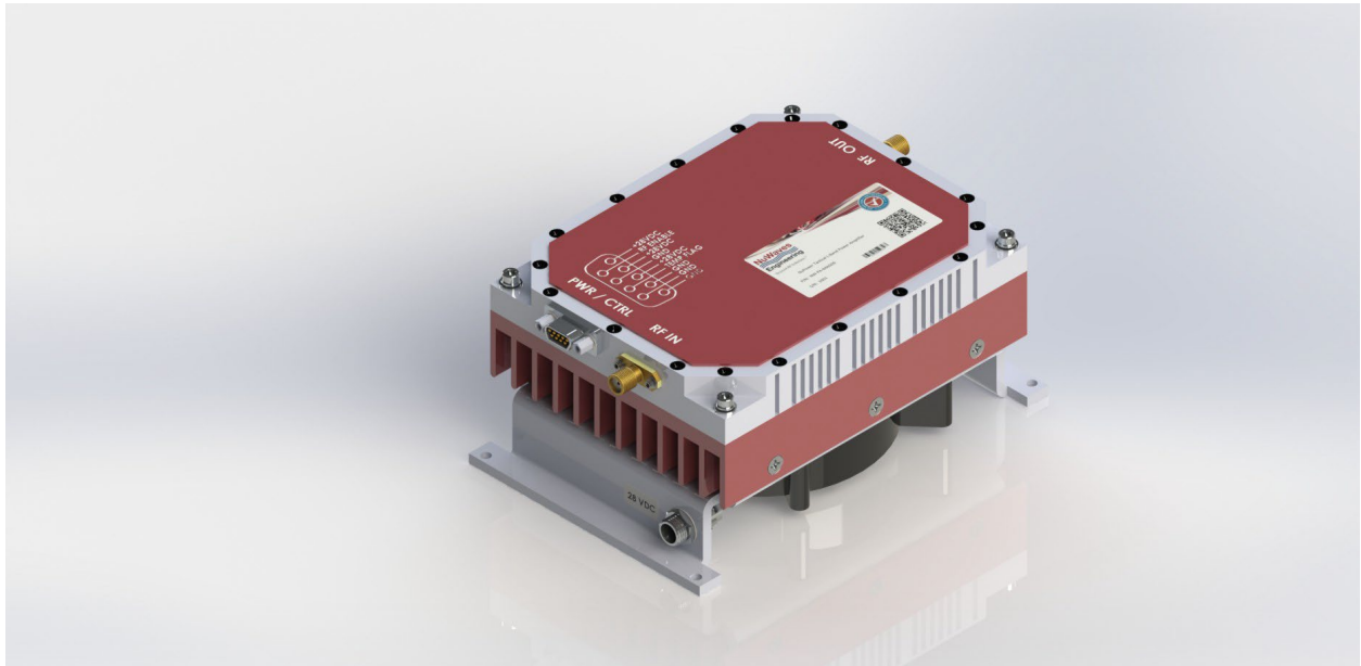
Figure 3: The NuPower PA Kit offers “out-of-the-box” operation for the user. The 28 VDC fan-cooled heatsink is shown with the NuPower 05E05A mounted.
