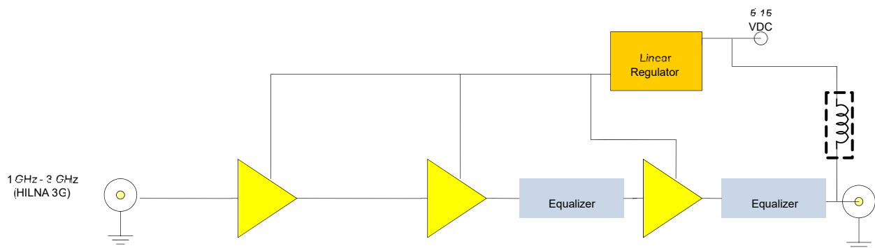
Figure 1: HILNA LS Functional Diagram
