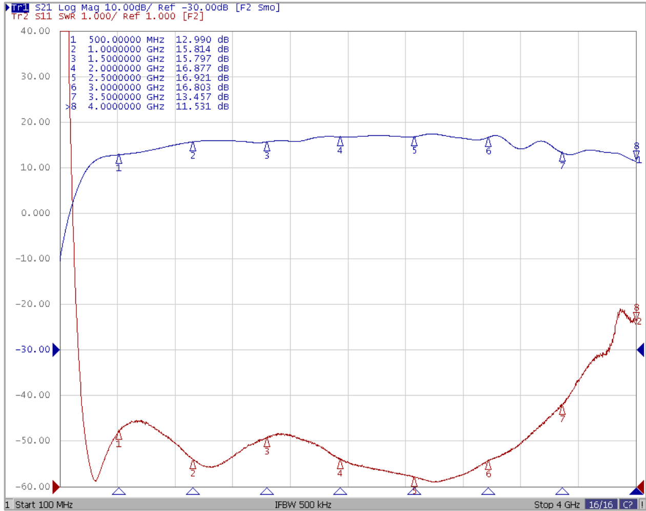
Figure 2: HILNA LS-C021-D Frequency Response
