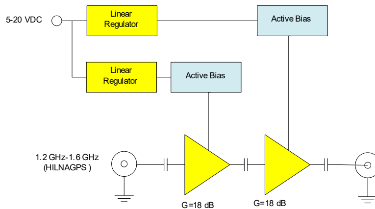
Figure 1: HILNA GPS Functional Diagram
