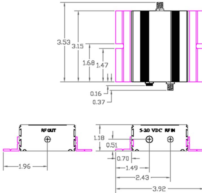
Figure 3: HILNA GPS Mechanical Outline
