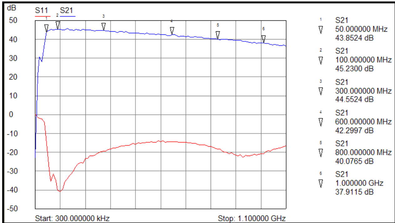
Figure 2: The HILNA G2V1 provides 40 dB (typ) of gain across the frequency range of 50 to 1000 MHz.
