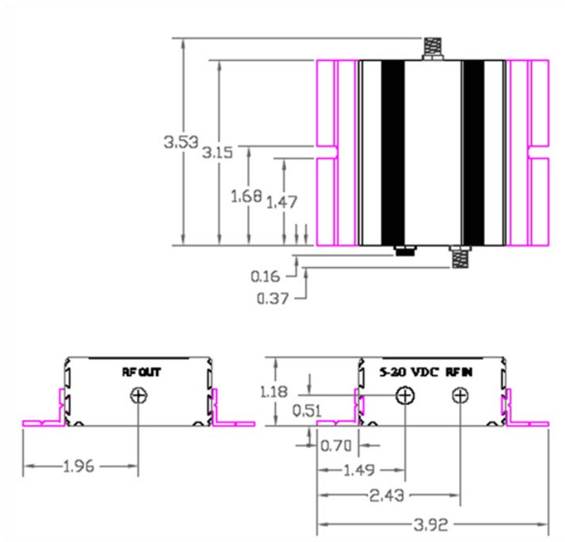
Figure 3: HILNA G2V1 Mechanical Outline
