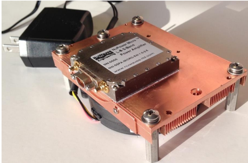
Figure 3: The NuPower PA Kit offers “out-of-the-box” operation for the user. The fan-cooled heat sink with an AC/DC adapter is shown with an example PA (NuPower LS5MI01-D30 not shown).
