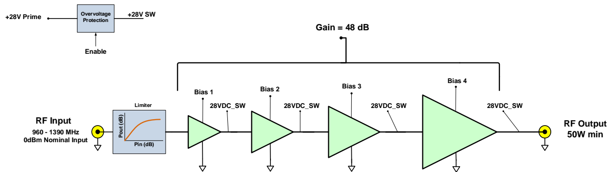
Figure 1: NuPower L60T01 Functional Diagram
