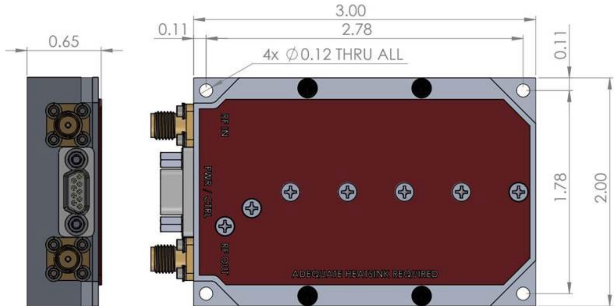
Figure 2: NuPower Xtender LS20S01-D19 Mechanical Outline
