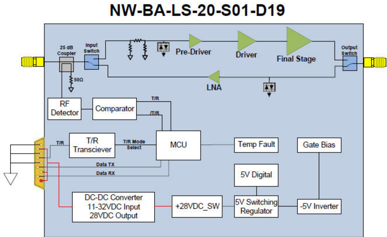
Figure 1: NuPower Xtender LS20S01-D19 Functional Diagram
