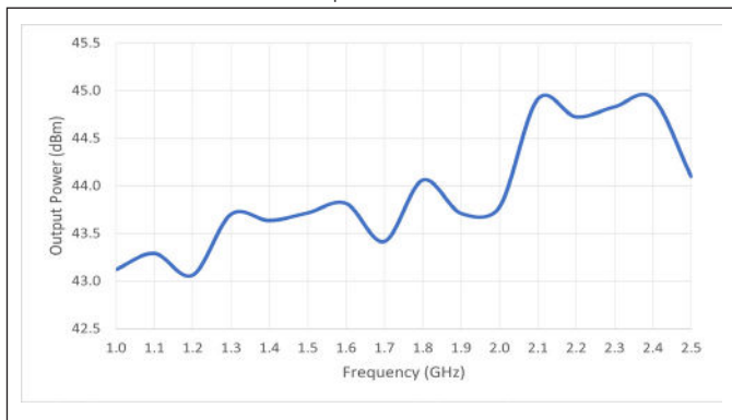
Output Power
