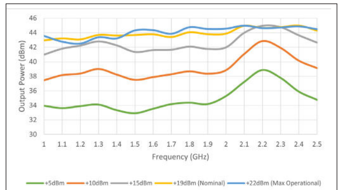
Output Power - Stepped Input Power
