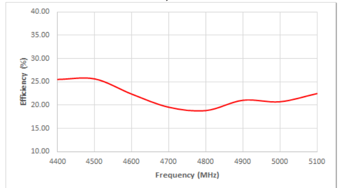
Efficiency - C-Band
