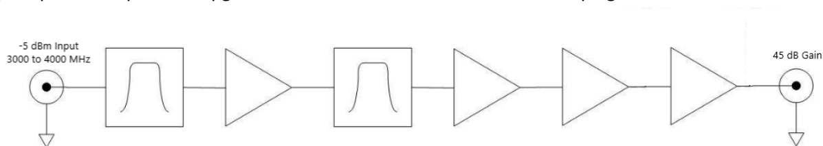
Figure 1: NuPower NW-PA-S-10-C01-S01 Functional Diagram
